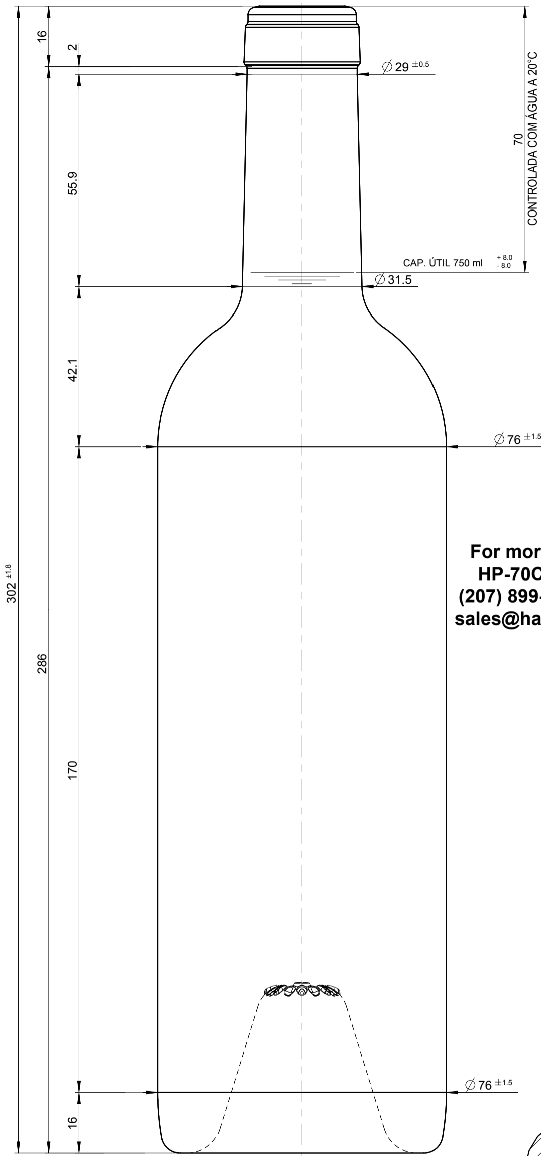
VISTA FRONTAL / FRONT VIEW
